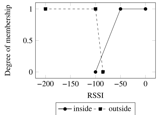
Fig. 4. Fuzzy membership functions to determine closeness as a function of RSSI value.
