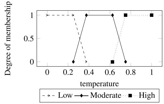
Fig. 5. Example of automatic execution with 3 default intervals.
