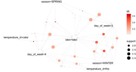
Fig. 12. Graphical representation of the rules obtained in the form of a graph.
