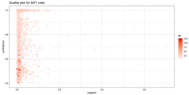
Fig. 14. Association rules generated by the traditional fusion method.
