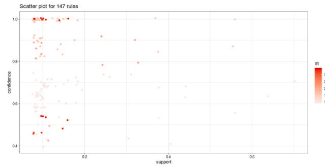
Fig. 15. Association rules generated by the fuzzy fusion method.
