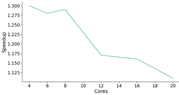
Fig. 7. Speed up of algorithm.
