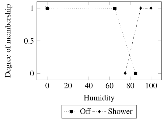
Fig. 8. Example of fuzzy-labels of the shower sensor.
