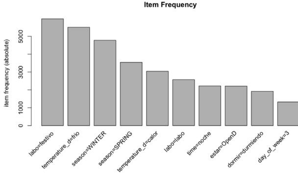
Fig. 9. Demonstration of most frequent elements with the standard fusion, illustrating a high incidence of unused or inactive sensors.
