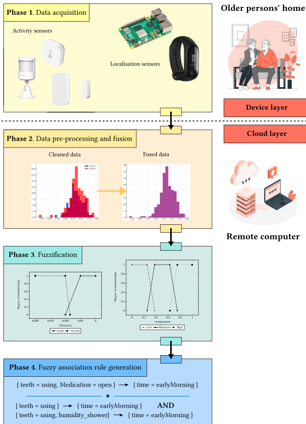
Fig. 1. Summary of the system workflow which has been divided into four main phases.
